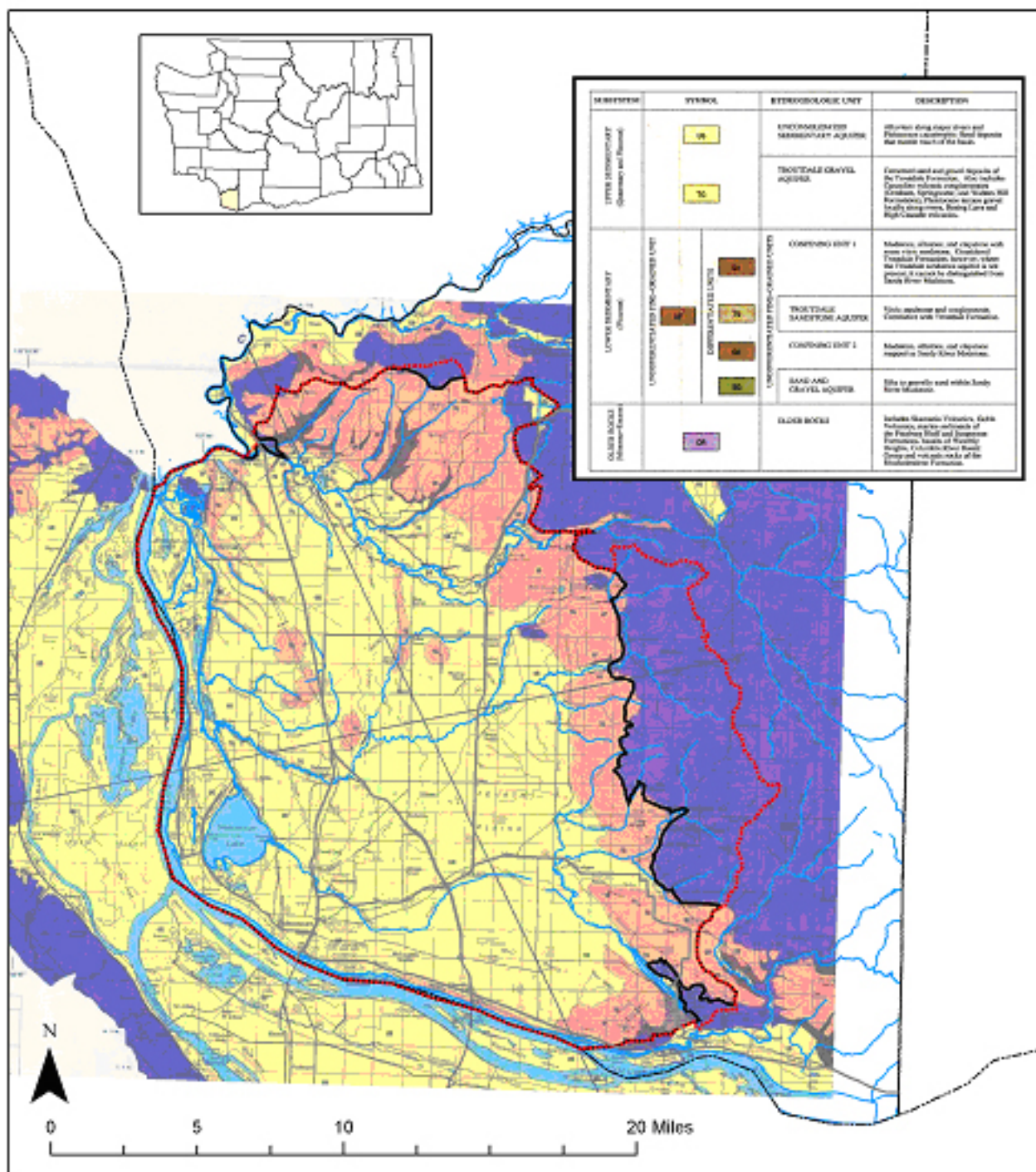
Figure 4: Hydrogeologic Map of Area (map image and key taken from Swanson, et al. 1993)
